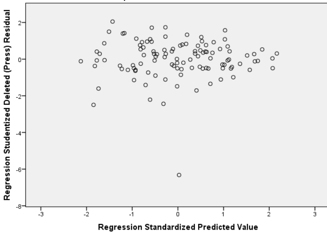
Figure 1. Scatterplot for Predicted GPA Scores and Regression Residuals
